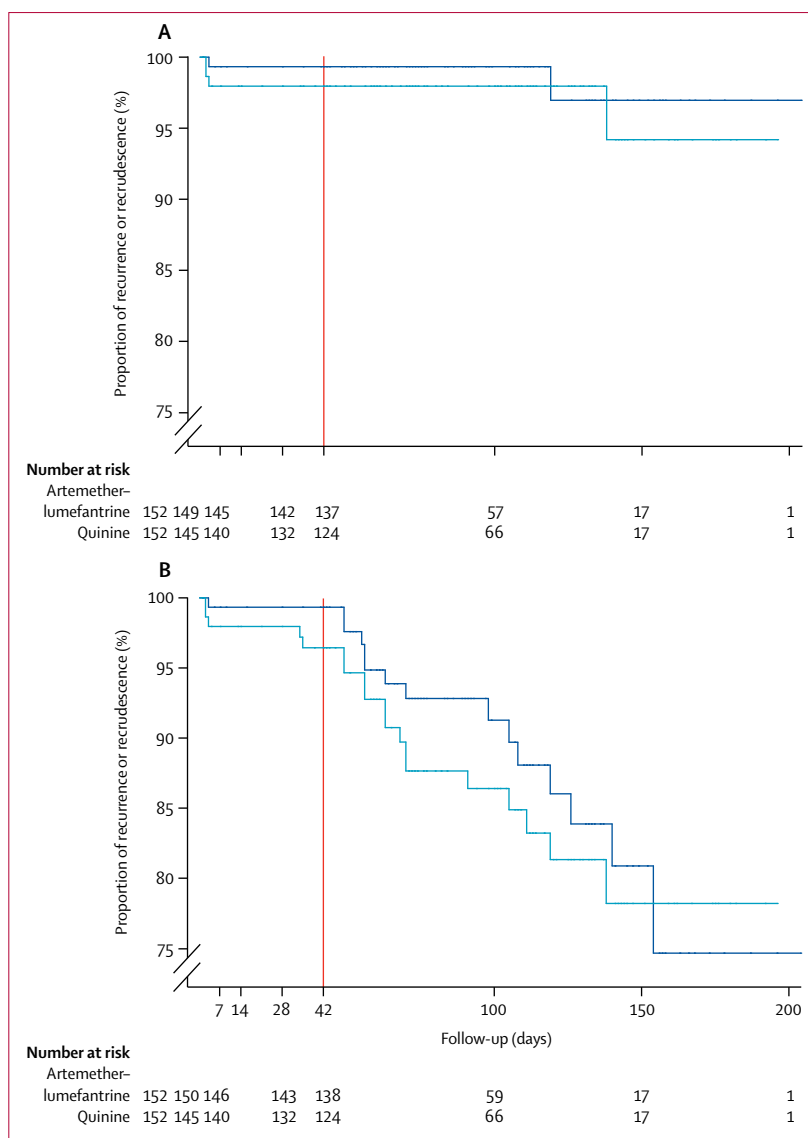
Figure 2: PCR-adjusted and unadjusted survival curve
