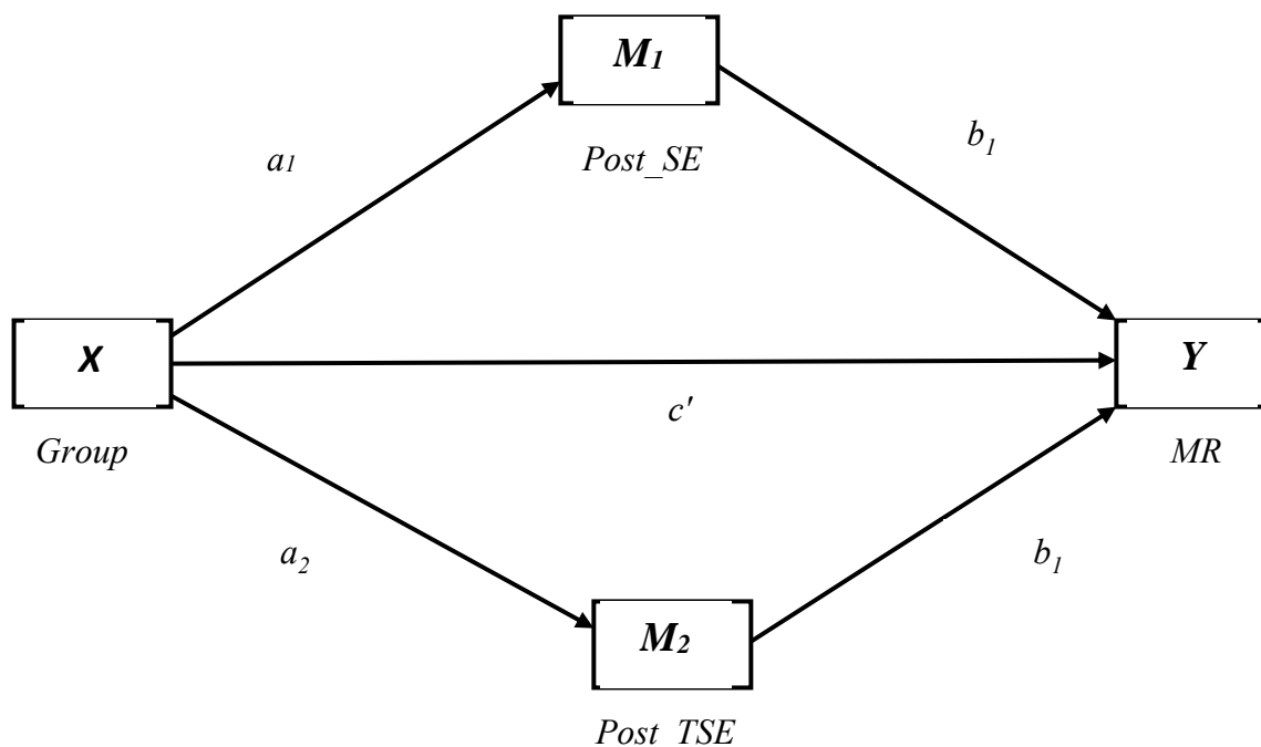
Figure 1. A Conceptual Diagram of a Parallel Multiple Mediator Model (adapted from Hayes, 2018, p.150).
