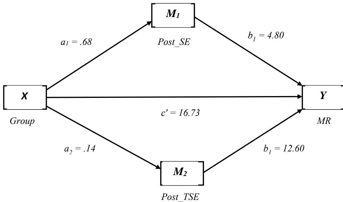
Figure 2. Parallel Multiple Mediator Model for the Teaching Method (Group), Self-Efficacy (M 1 &M 2 ) and Mathematical Reasoning (MR)
